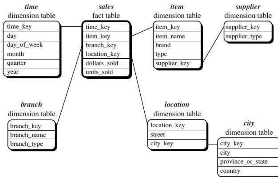
Figure 10.10 Snowflake schema of a data warehouse for sales.
